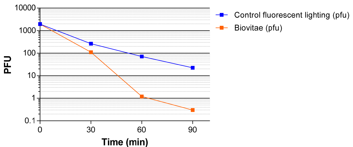
Fig 8: Evolution of the number of residual infectious particles (PFU) after irradiation at different times with the Biovitae® lamp and the control fluorescent lighting
