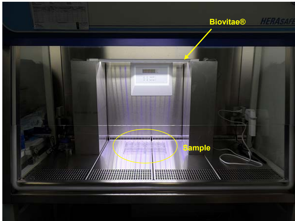
Fig 5: Dried viral samples placed under the Biovitae® lamp in a biosafety cabinet.
