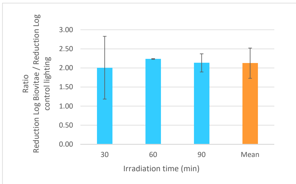
Fig 10: Ratio of the logarithmic reduction measured with Biovitae® on that measured with the control lighting for the different times tested (blue bars) and averaged over all times (orange bar).
